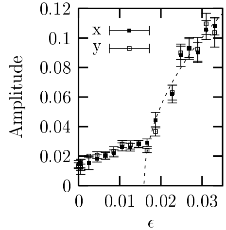
Fig. 11. Undulation amplitude as a function of the dilation \epsilon . For values of the dilation of \epsilon \approx 0.019 the system starts to respond with undulations and the amplitude increases continuously until the layers break apart for \epsilon > 3\% . The dashed line (---) shows a fit to the data points assuming a square root dependence of the amplitude above onset.
